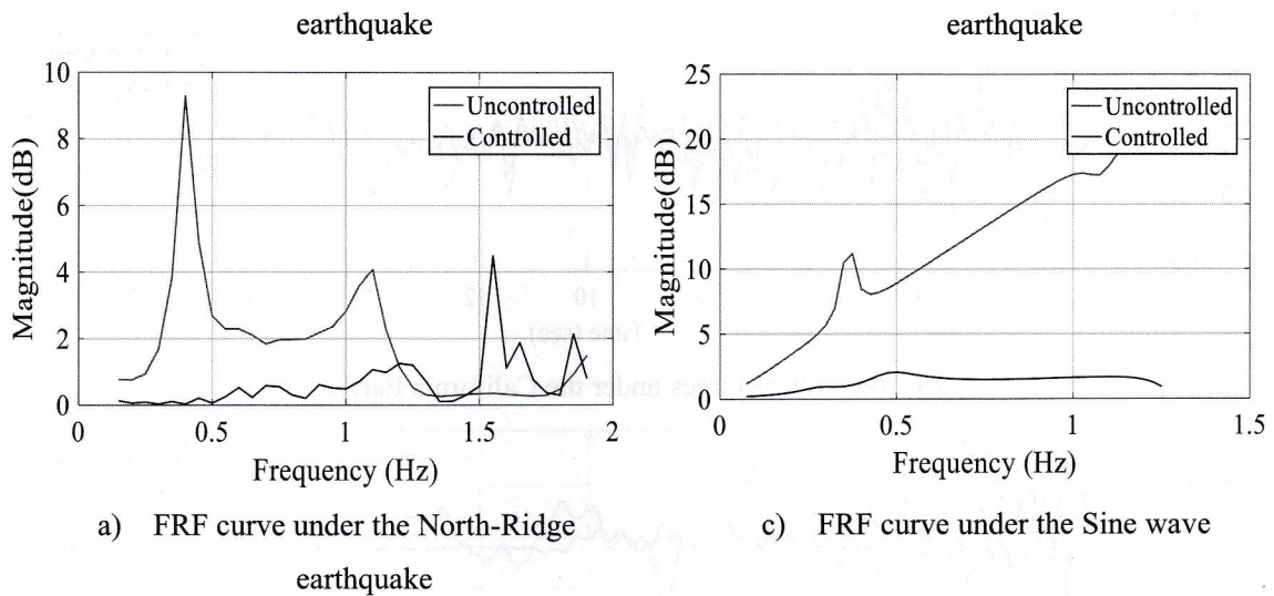
Fig.8: Frequency response curves under different excitations
