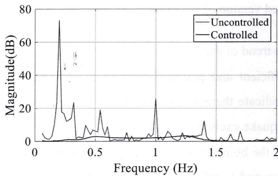
a) FRF curve under the El-Centro
