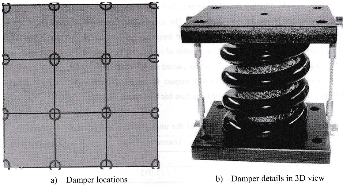
Fig.3: Spring damper device locations and details
