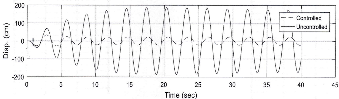
Fig.5: Top floor Displacement under the Sine wave signal with frequency 0.3382 Hz
