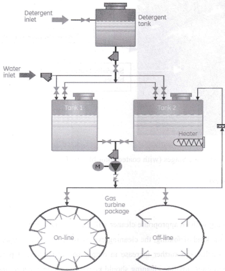
Fig.3 :Pictorial Representation of water wash system[14]
