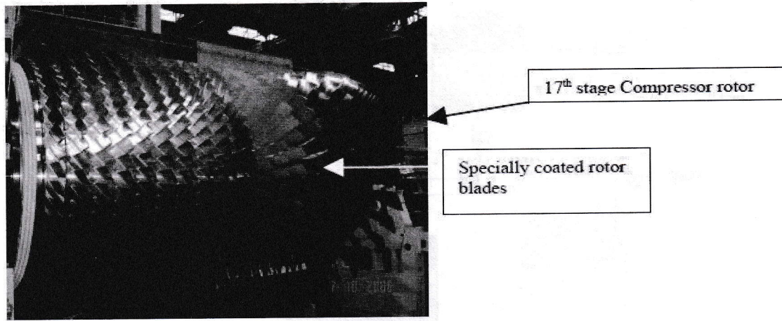
Fig.2: Compressor Stages (with coated rotor blades) [11]
