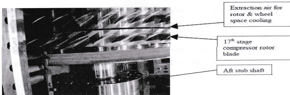
Fig.1:Compressor Stages[11]
