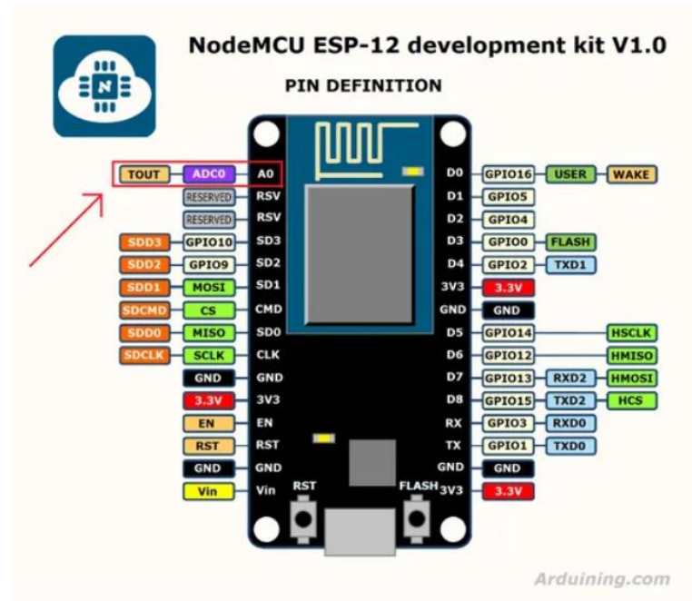
Fig 3.7 Pinout-Analog [13]
