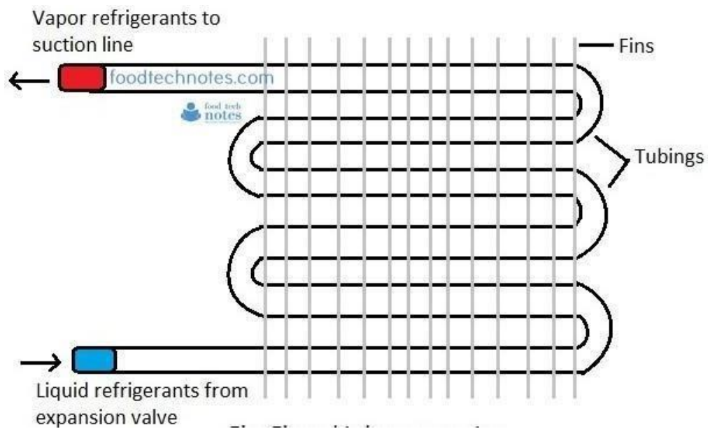
Figure 5.7: Finned Tube Evaporator
