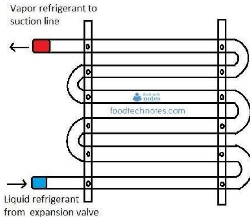
Figure 5.5: Bare Tube Evaporator
