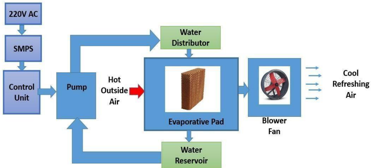
Figure 4.1: Block Diagram of Evaporative Cooling System.
