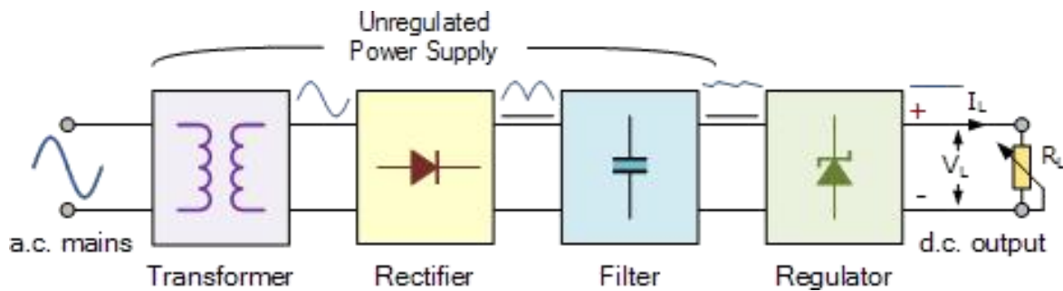
Figure 5.4: DC Power Supply Step
