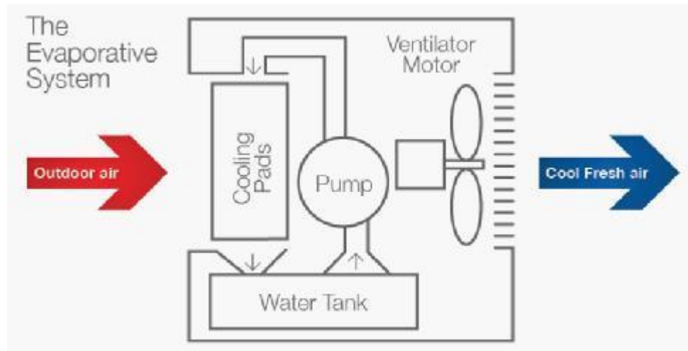
Figure 3.2: Working Principle of Evaporator Cooling System
