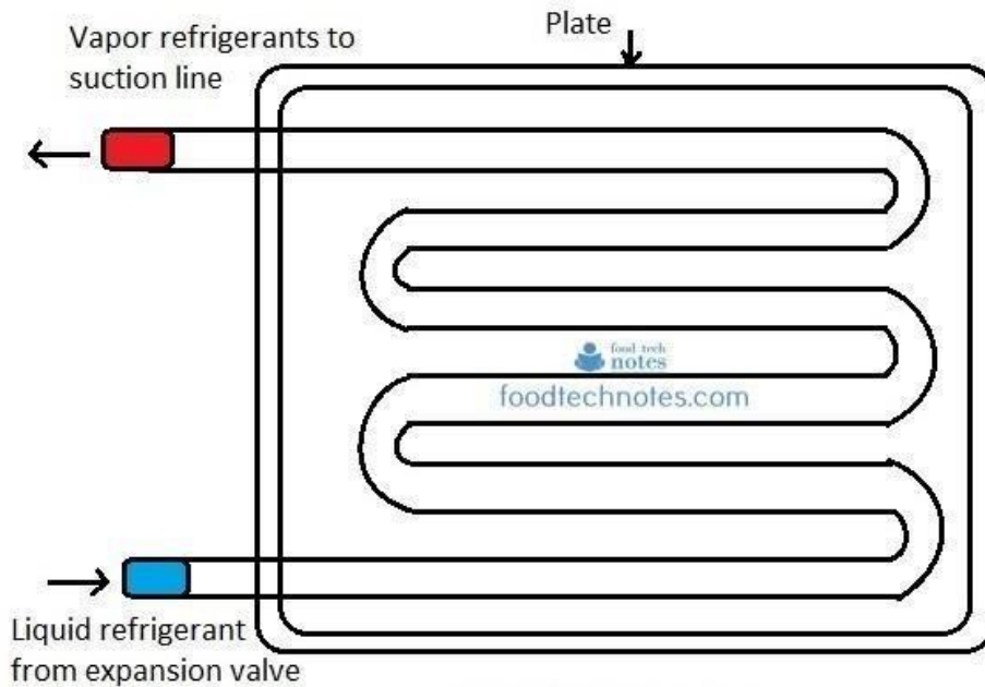
Figure 5.6: Plate Evaporator
