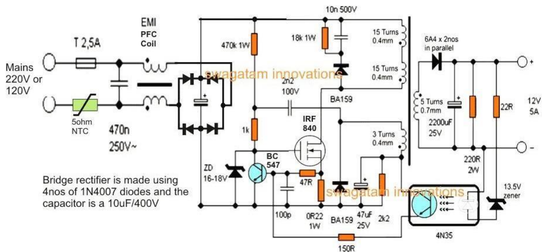
Figure 5.2: SMPS Circuit Design
