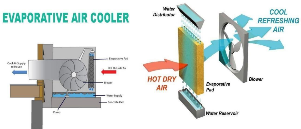
Figure 3.1: Evaporator Cooling Working Principle..
