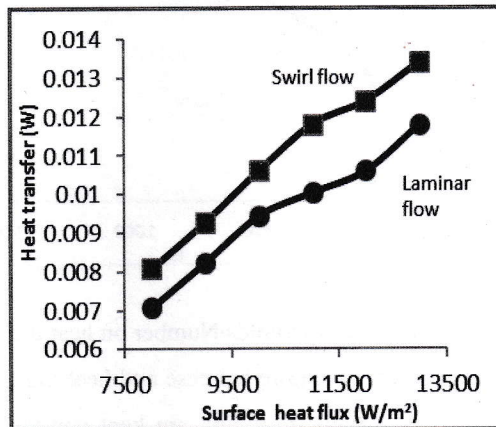
Fig. 10. Heat transfer with surface heat flux.
