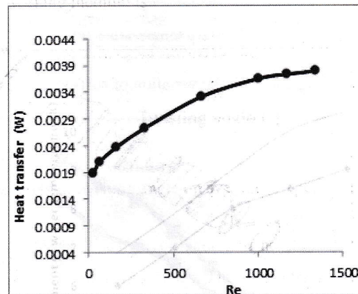
Fig. 12. Effects of Reynolds Number on heat transfer.
