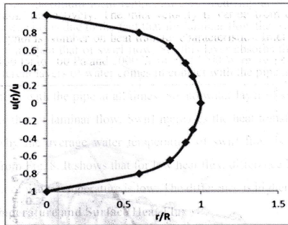
Fig. 5. Velocity profile obtained from numerical study.
