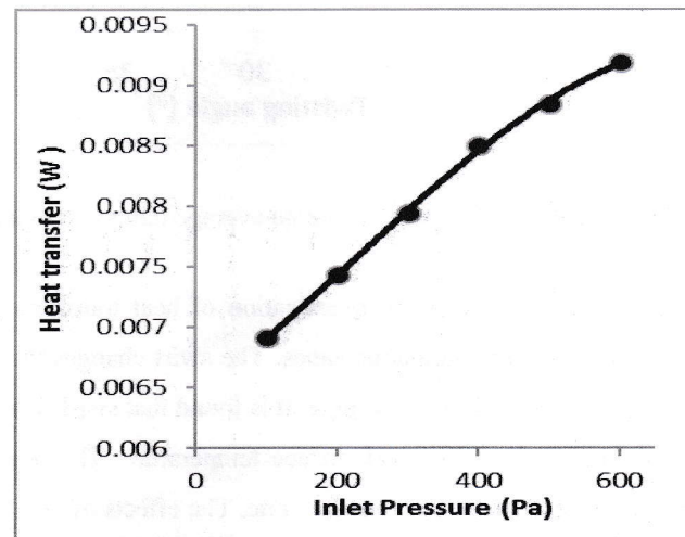
Fig. 14. Effects of inlet pressure on heat transfer.
