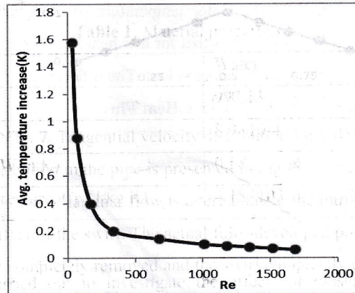
Fig. 11. Effects of Reynolds Number on flow temperature.
