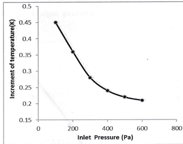
Fig. 13. Effects of inlet pressure on temperature increase.
