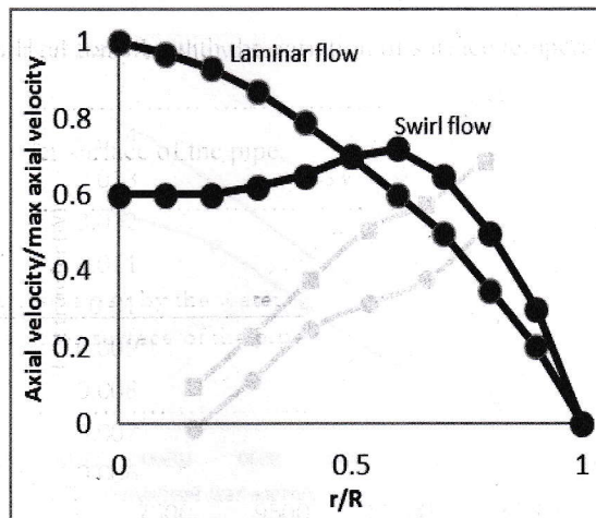
Fig. 6. Radial velocity distribution for x/d=5 .
