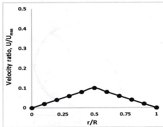
Fig. 7. Tangential velocity distribution for x/d=5.
