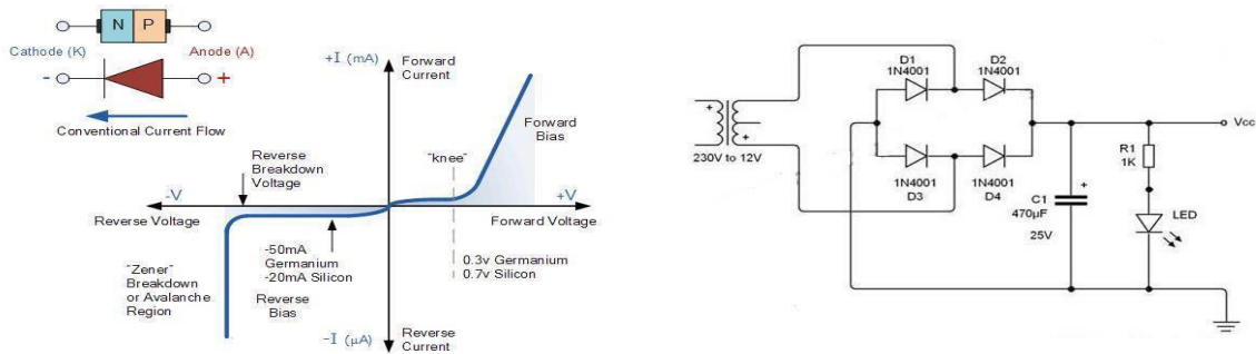
Figure 4. 7 Junction diode symbol and static I-V characteristics
