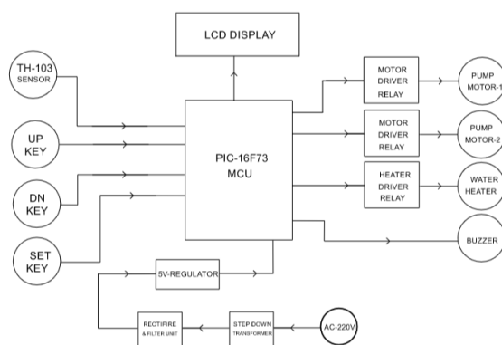
BLOCK DIAGRAM :BOILER WATER TEMPERATURE AND FLOW CONTROL AND MONITORING SYSTEM
