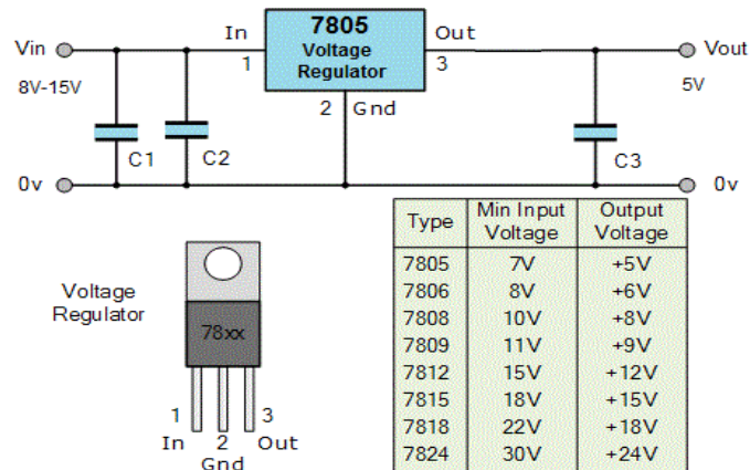
Figure 4. 12 Voltage regulator output voltages.
