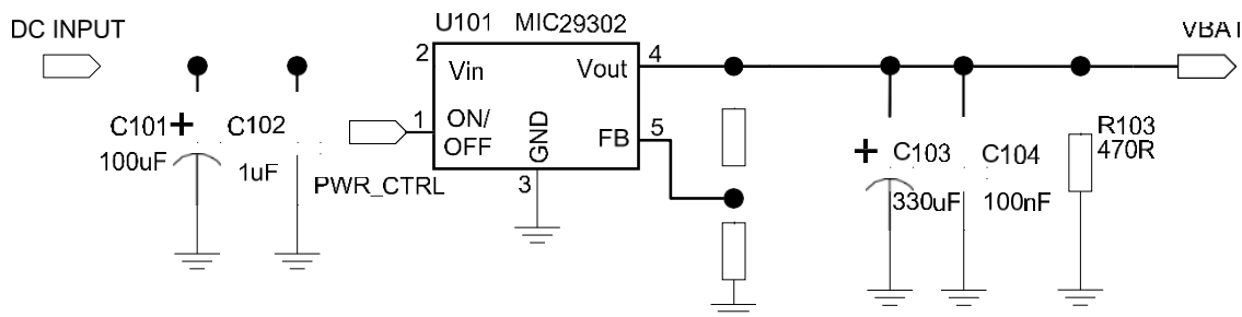
Figure 4. 14 Reference circuit of the DC-DC power supply
