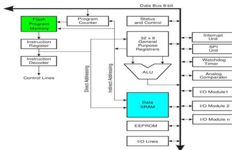
Figure 4. 2 Arduino Architecture:
