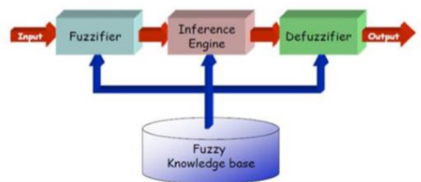
Fig.6. Block diagram of fuzzy inference system
