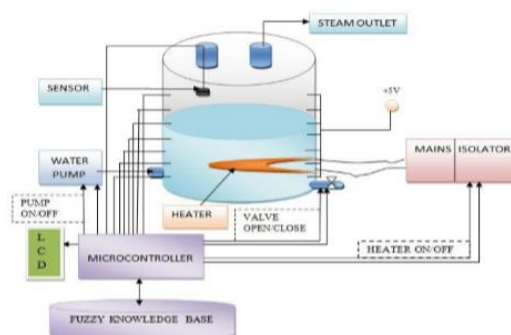
Fig.2. Proposed FLC based boiler control
