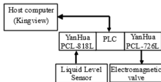
Fig. 3. Hardware of control system
