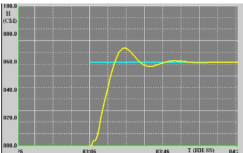
Fig. 6. The operation results while KP=2 , KI=1.5
