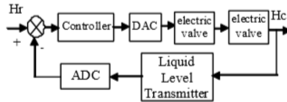
Fig. 2. Structure of level control system
