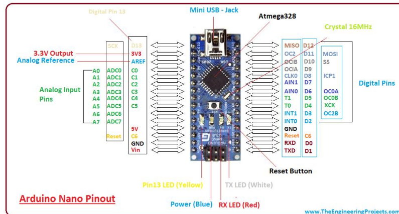
Figure 4.3: Arduino pin diagram
