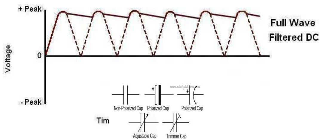
Fig. 3.10 Filtered output
