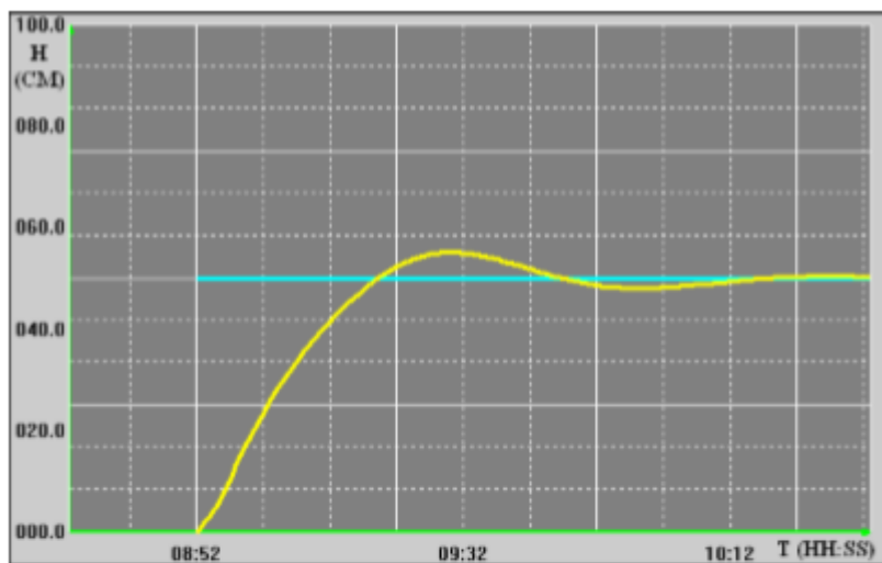
Fig. 5. The operation results while KP=1 , KI=0.7
