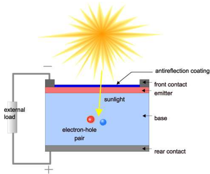
Figure 3.4: Solar Panel Schema Diagram
