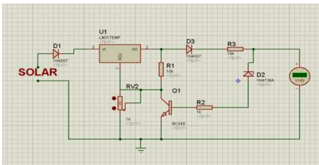
Figure 3.7: Solar Charger Controller Circuit
