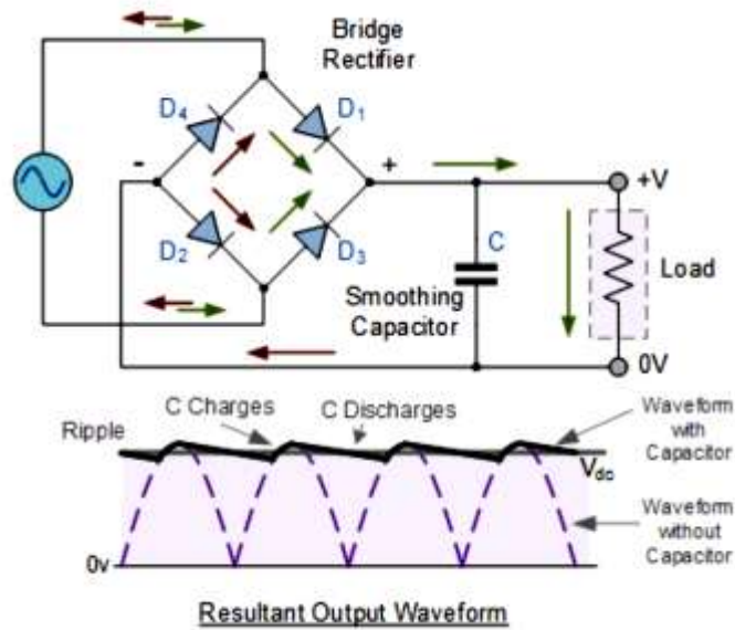
Figure 3.10: The Smoothing Capacitor with Full Bridge Rectifier
