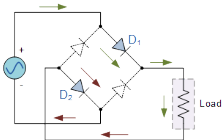
Figure 3.4: The Positive Half-cycle
