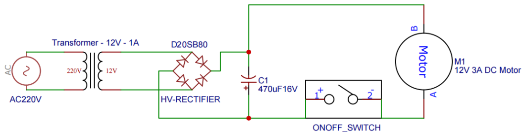
Figure 4.3: Schematic Diagram of the Project
