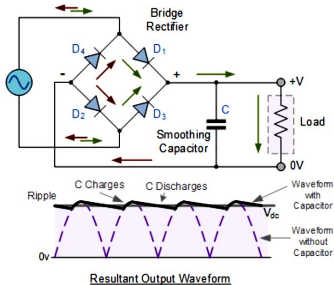
Figure 3.7: The Smoothing Capacitor with Full Bridge Rectifier
