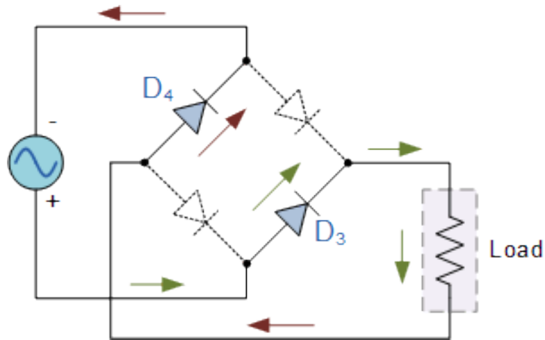
Figure 3.5: The Negative Half-cycle
