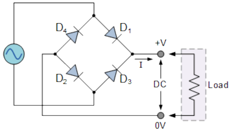
Figure 3.3: The Diode Bridge Rectifier
