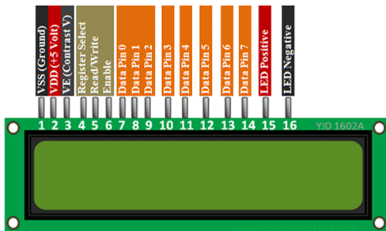
Figure 3.10 16x2 LCD connection
