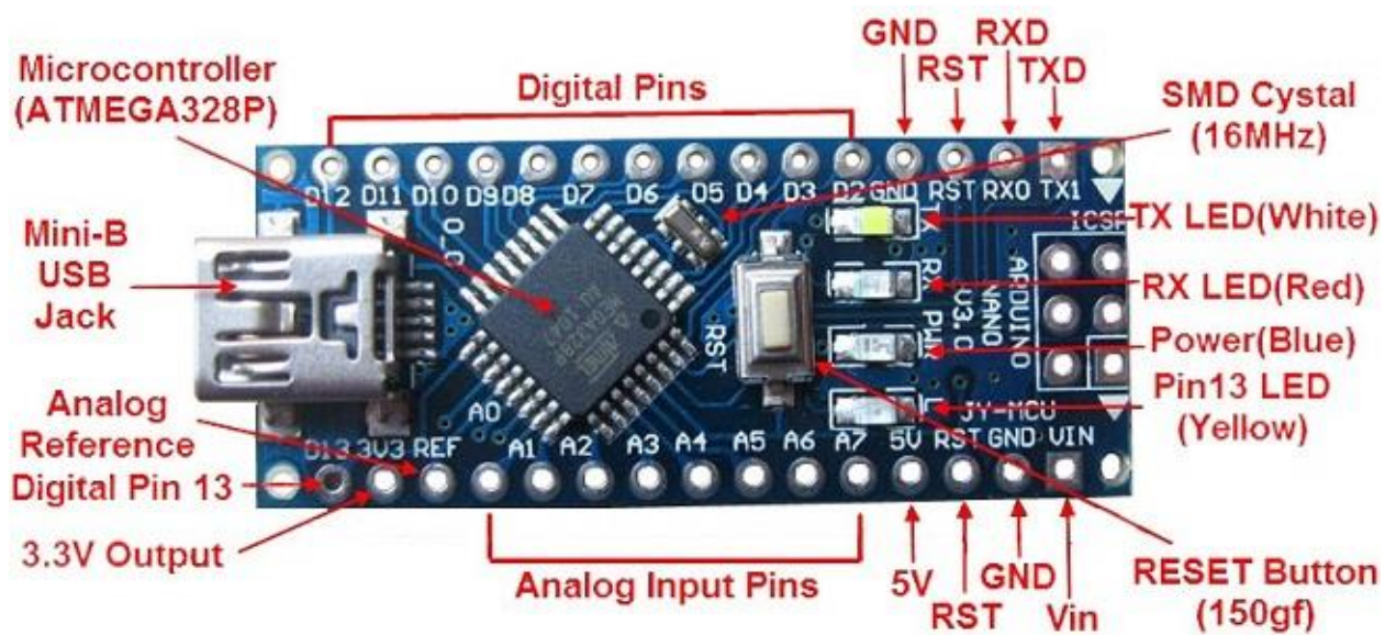
Figure 3.1: Arduino Nano
