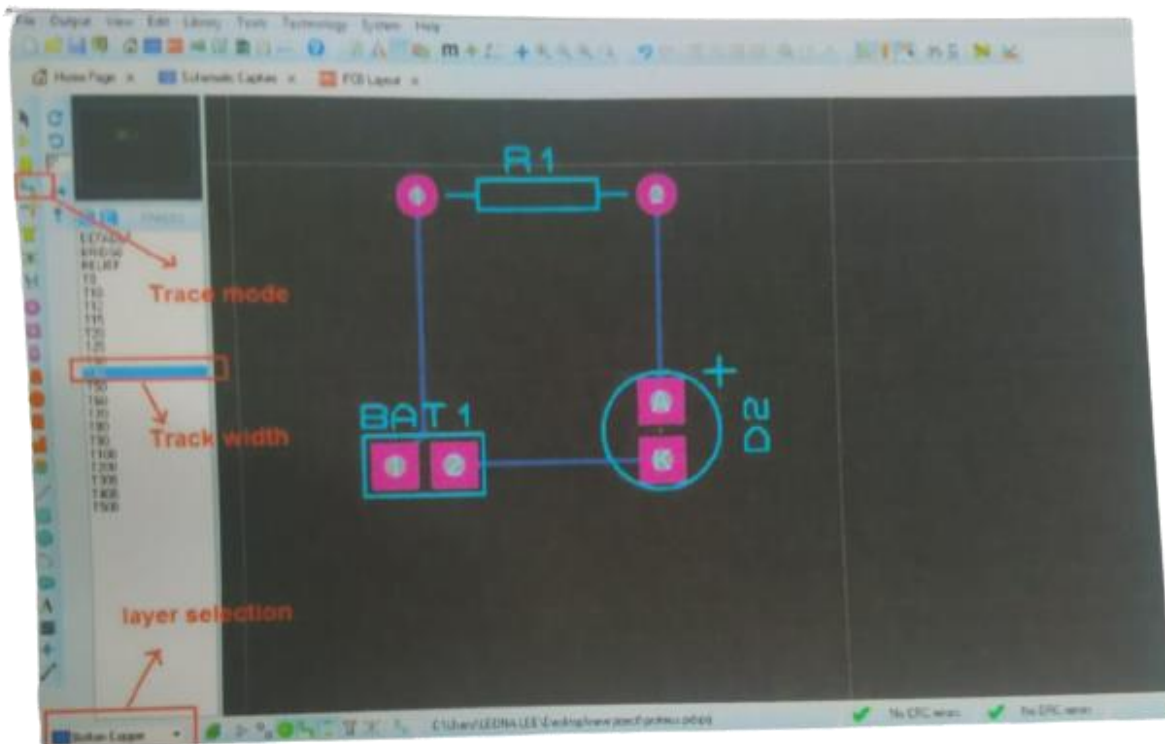
Figure 4.3: PCB Design
