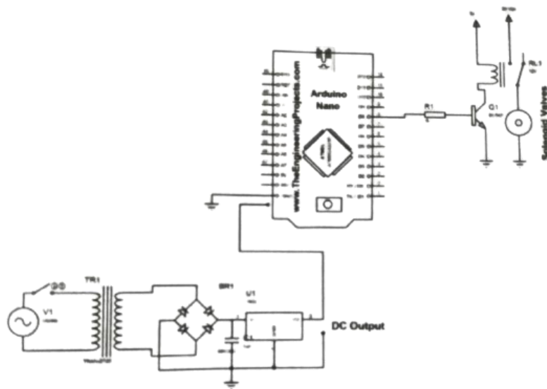
Figure 2.3: Circuit Diagram of Project [2]
