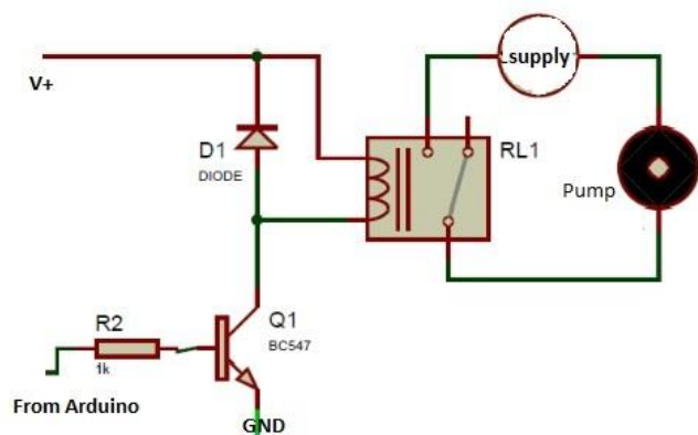
Fig 3.5: Relay
