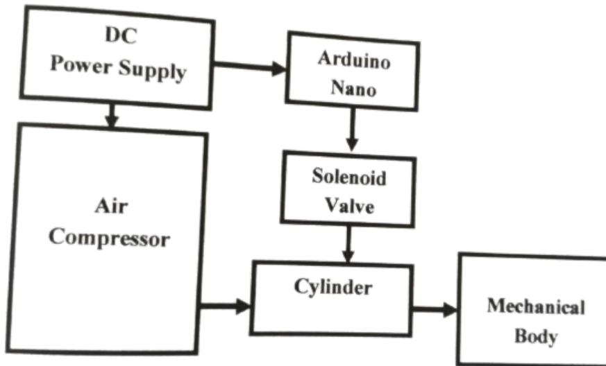
Figure 2.2: Block Diagram of Project
