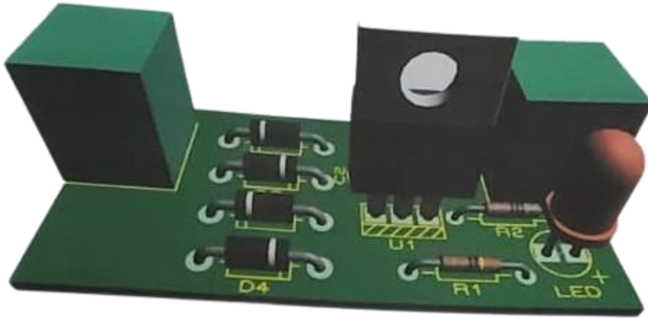
Fig 4.4: 3D verification
