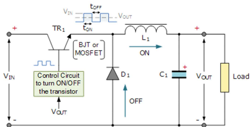
Figure 3.3 : SMPS Diagram [19]
