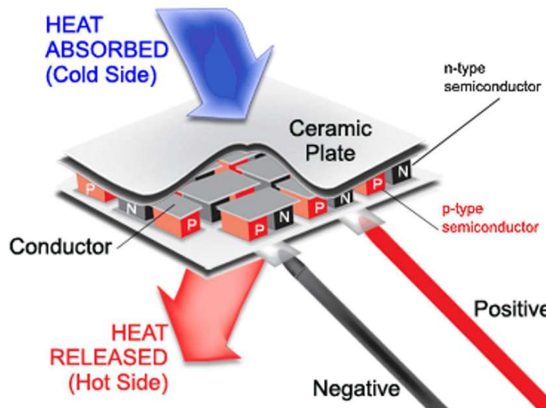
Figure 3.6 : Construction of Peltier [22]
