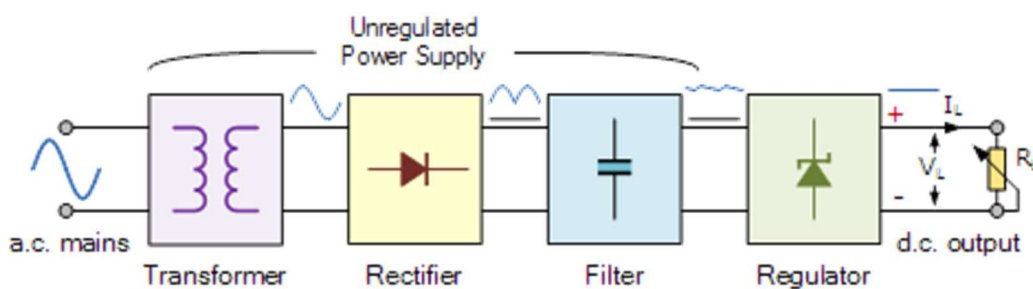
Figure 3.4: DC Power supply way [20]
