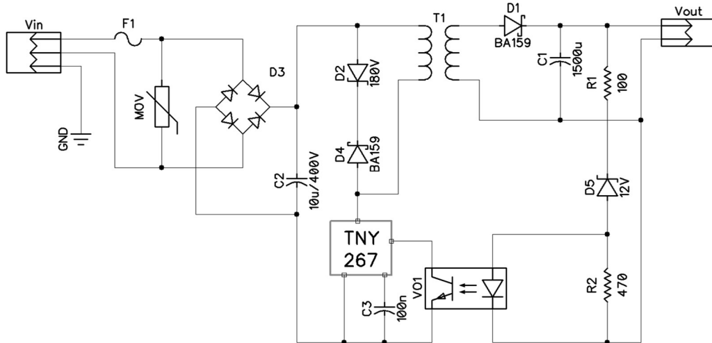
Figure 3.2: Basic working concept of an SMPS [18]
