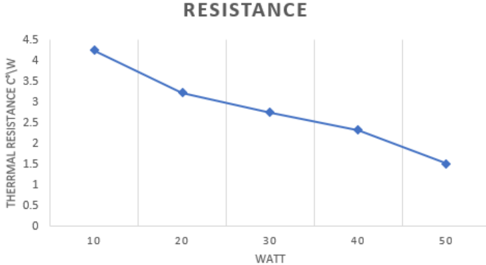
Figure 4-3 Thermal resistance vs heat input (Watt) 50% FR position 45 degree
