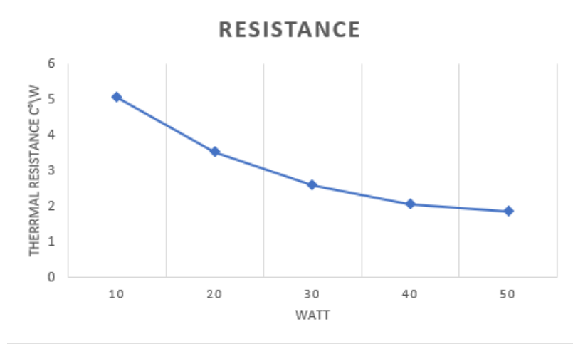
Figure 4-8 Thermal resistance vs heat input (Watt) FR 60% position 90 degree
