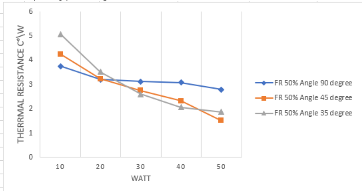
Figure 4-9 Thermal resistance vs heat input (watt) Ethylene glycol all
