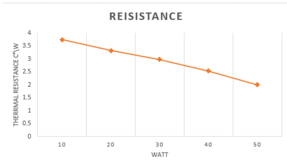
Figure 4-2 Thermal resistance vs heat input (Watt) 50% FR Position 90 degree
