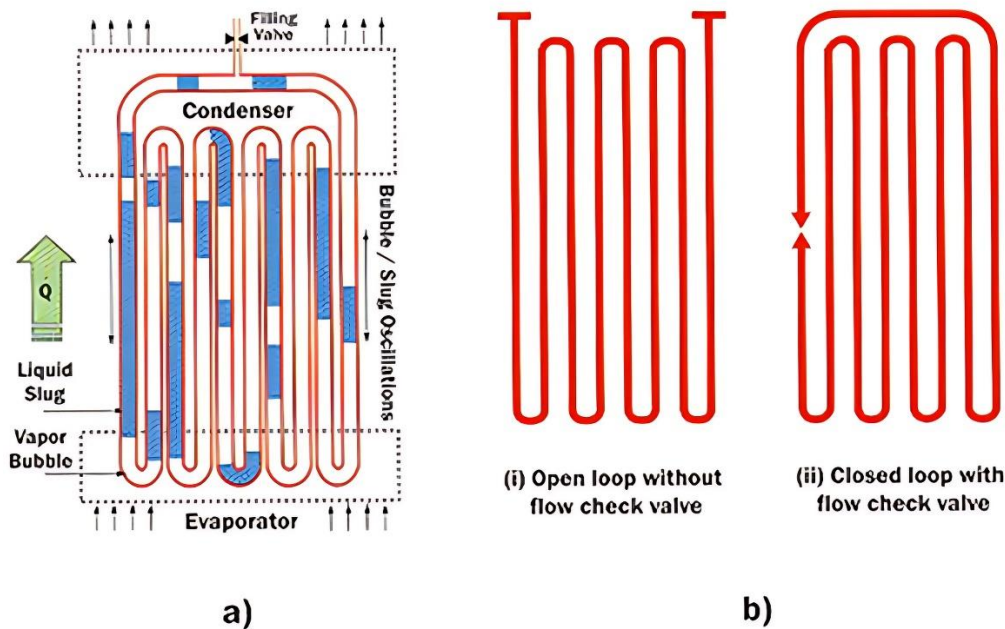
Figure 1-3 Types of CLPHP ( https://peregrinecorp.com/pulsating-heat-pipes/ )
