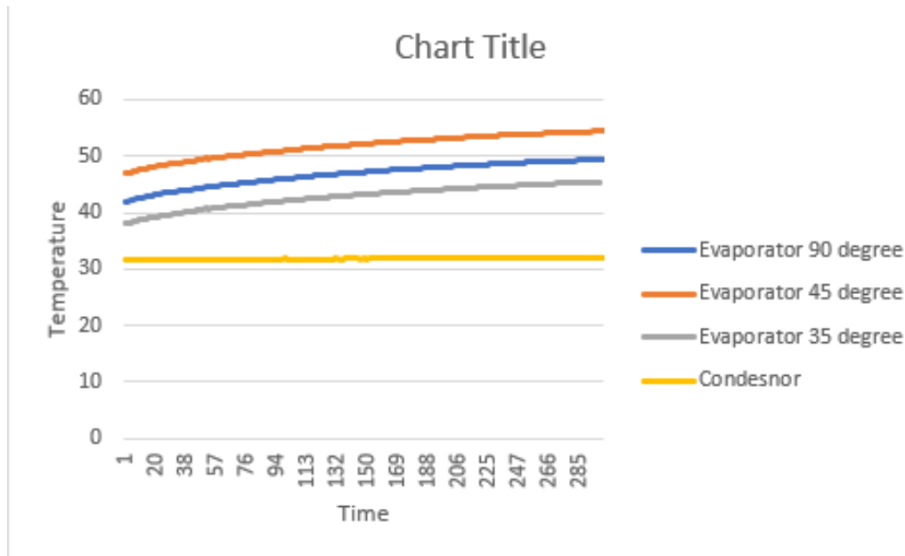
Figure 4-1 Heat vs Second Steady condition data Ethylene glycol
