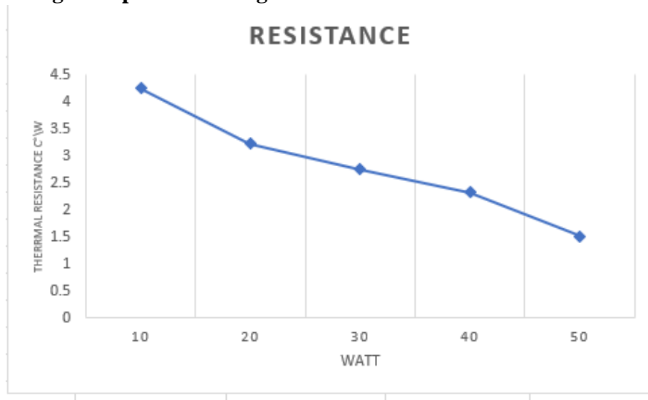
Figure 4-7 Thermal resistance vs heat input (Watt) methanol FR 50% position 45
