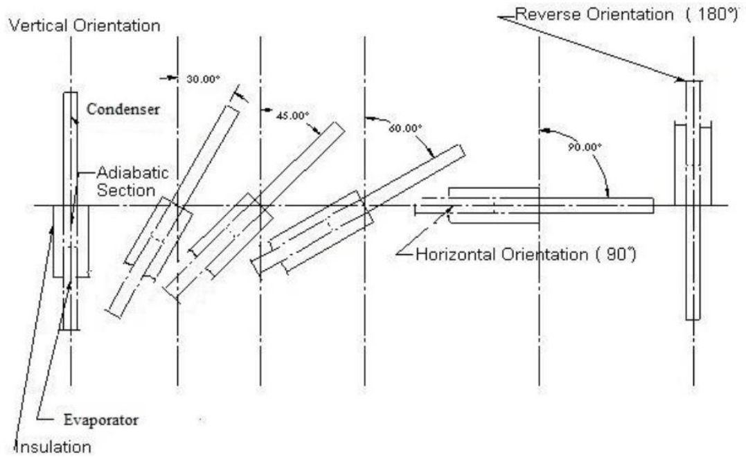
Figure 1-5 Angles hypothesis define origin in vertical plan
