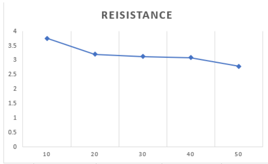
Figure 4-6 Thermal resistance vs heat input (watt) FR 50% position 90-degree Ethylene glycol
