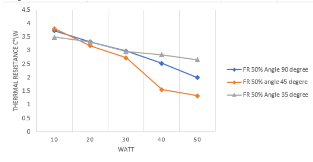
Figure 4-5 Thermal resistance vs Heat input (Watt) Methanol all
