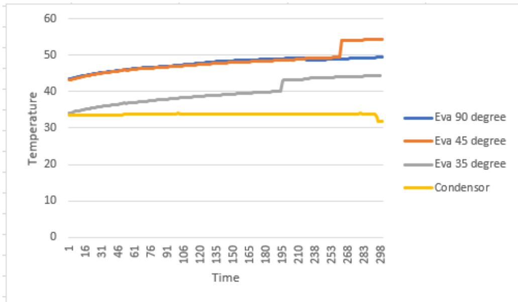
Figure 4-2 Heat vs Second Steady condition data Methanol
