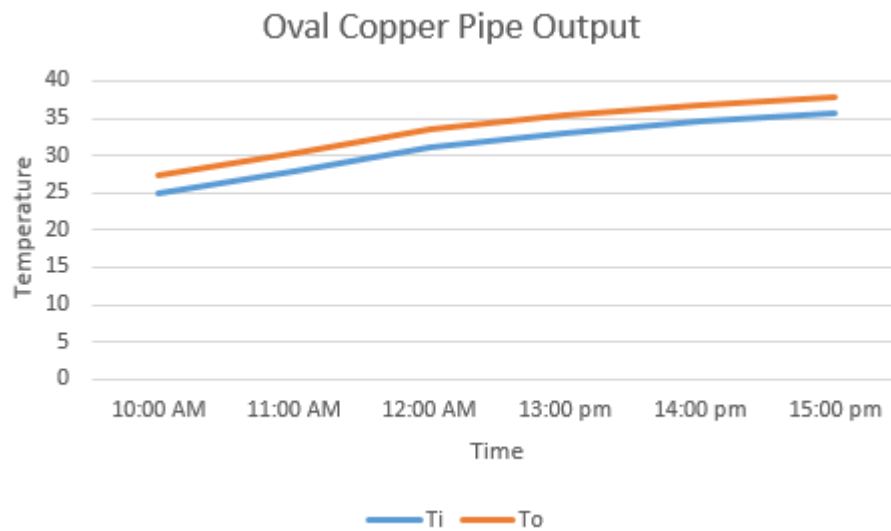
Graph 1.2: Temperature graph for Oval section Copper Pipe
