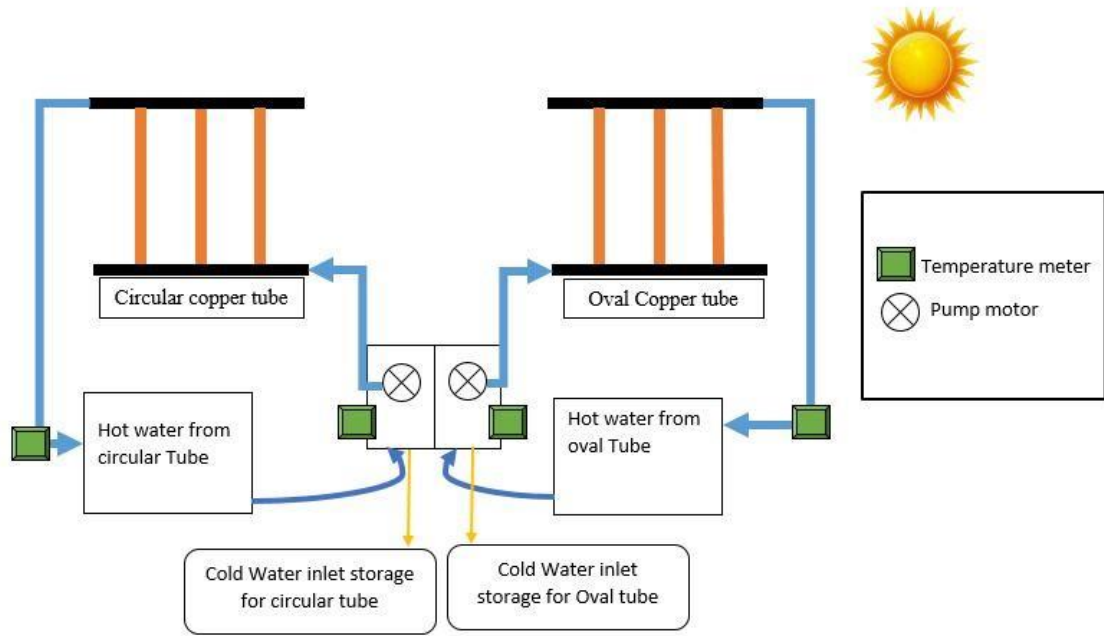
Figure 4.3: Structural Diagram of the project
