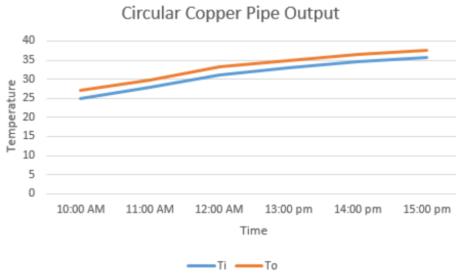
Graph 1.1: Temperature graph for Circular Copper Pipe
