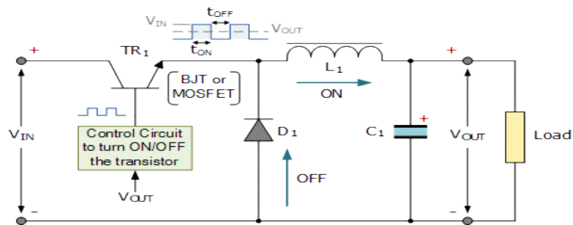
Figure 3.14: SMPS Circuit Connection
