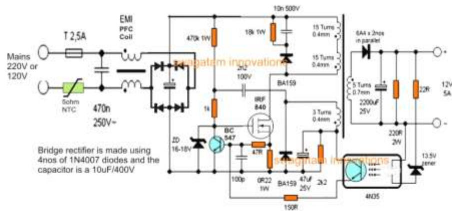
Figure 3.13: SMPS Circuit
