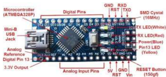
Figure 3.7: How Arduino Nano looks like
