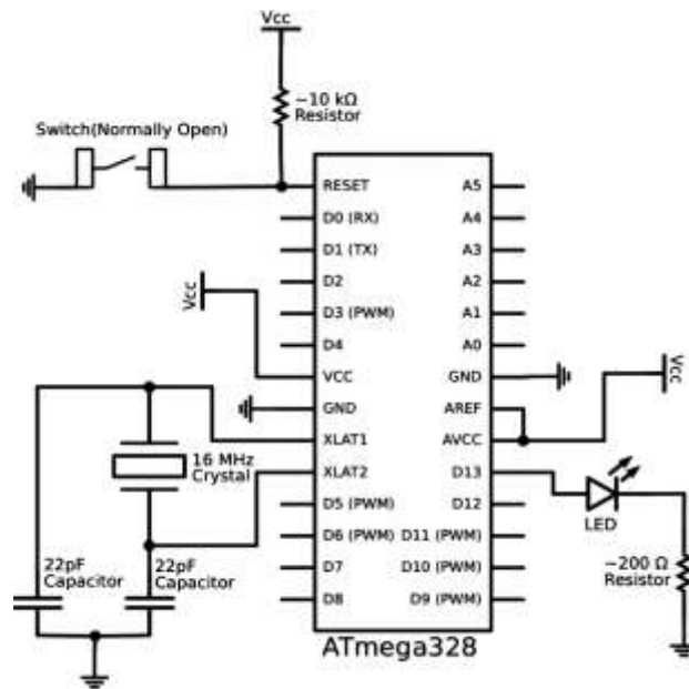
Figure 3.6: Arduino Nano Schematic Diagram
