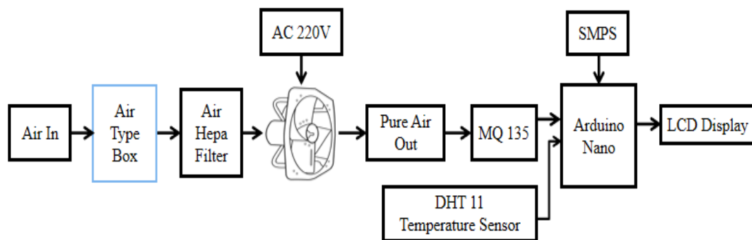
Figure 2.1: Block Diagram of Air Purifier and Air Quality Monitoring System
