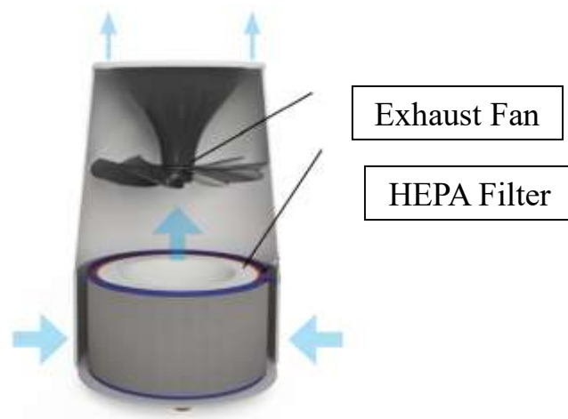
Figure 4.5: Our Final System Working Mechanism
