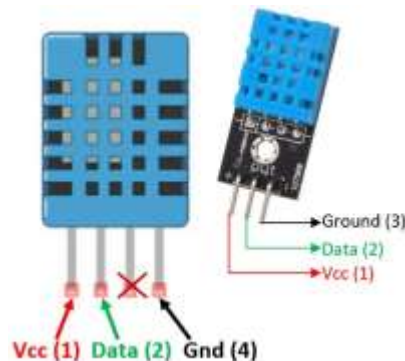
Figure 3.17: DHT11 Temperature Sensor
