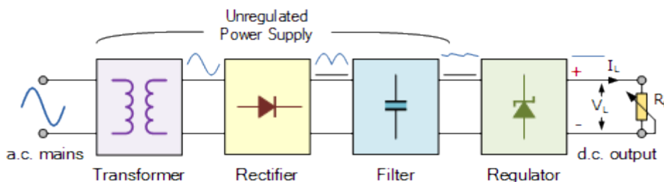
Figure 3.15: DC Power supply way
