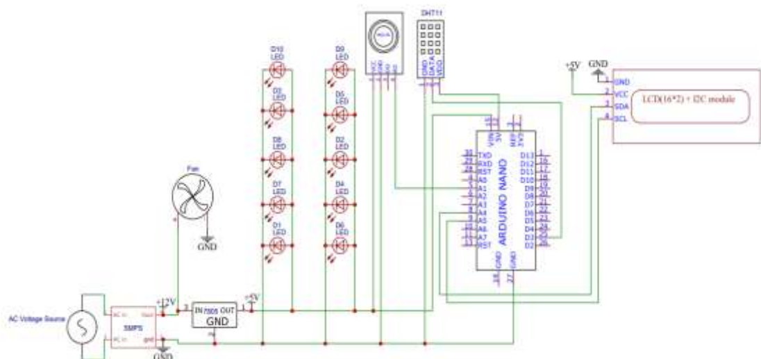
Figure 2.2: Schematic Diagram of our circuit
