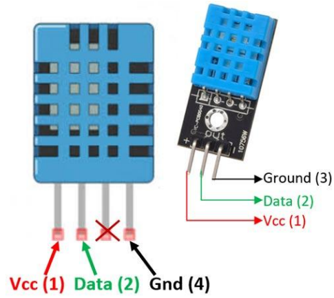
Figure 3.14: DHT11 Temperature Sensor
