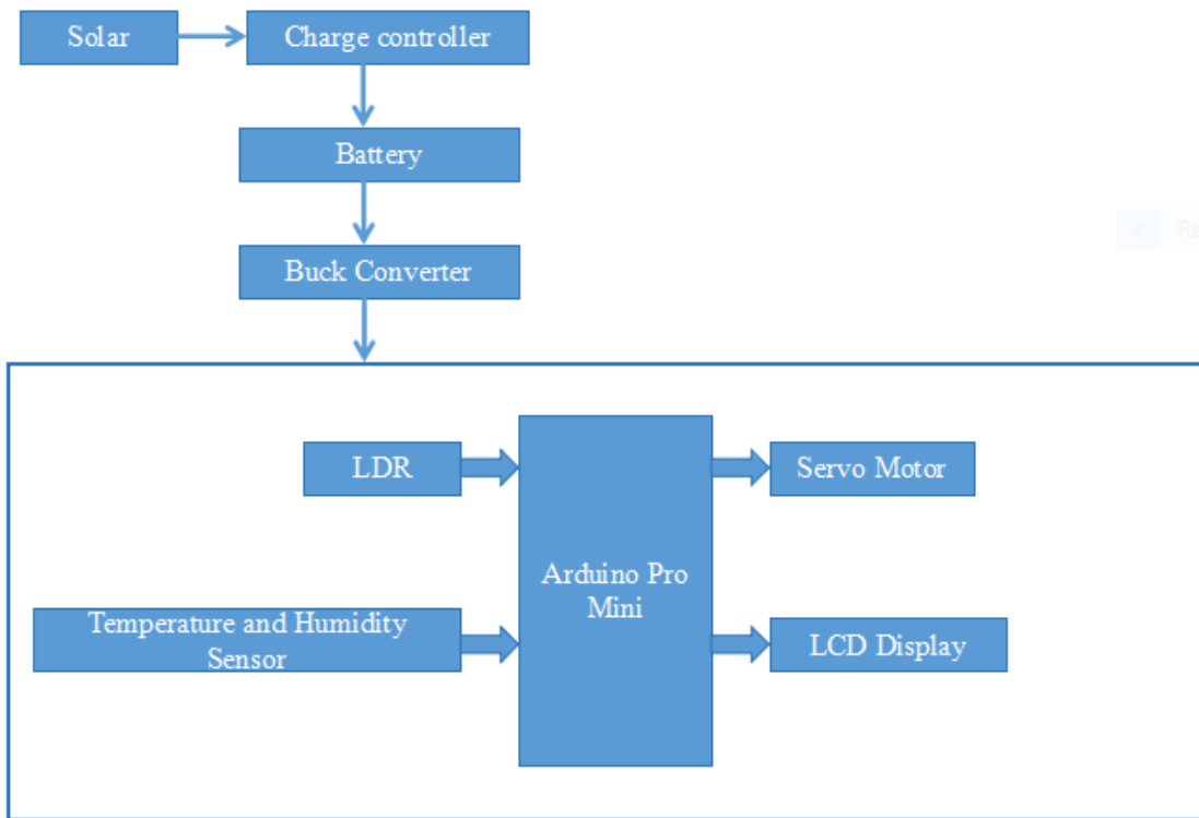
Figure 4.1: Block Diagram of our Project
