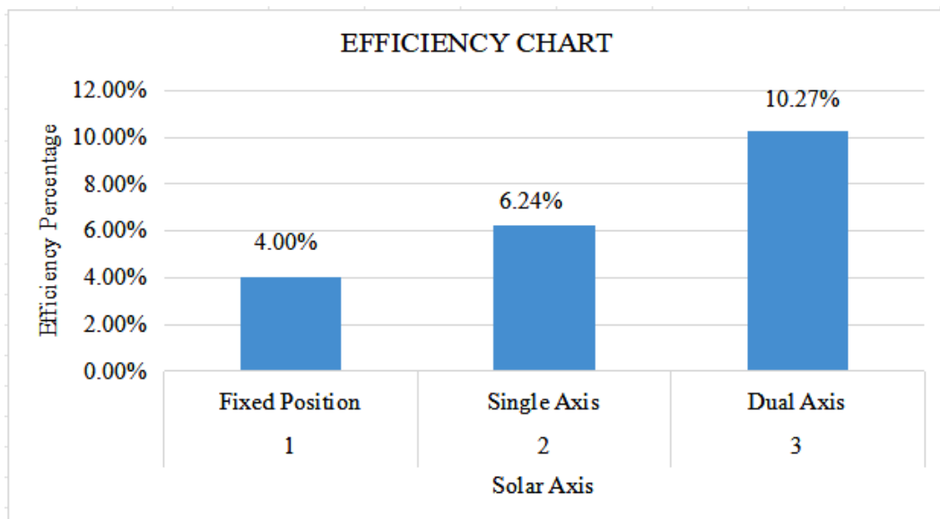
Figure 5.2: Efficiency Graph
