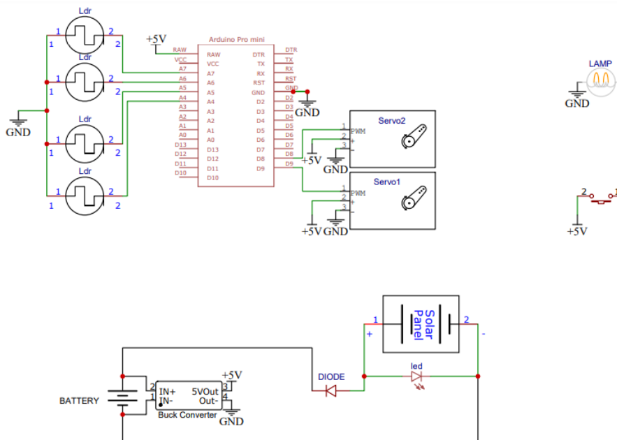
Figure 4.2: Circuit Diagram of Our System
