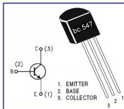
Figure 3.5: BC 547
