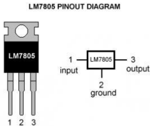
Figure 3.10: 5V Regulator IC
